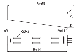
OBPHG 400/600
