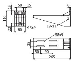
OBPHG 200
